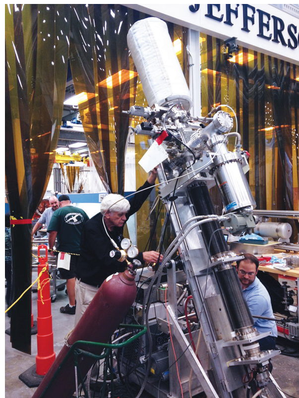
Larry Phillips (foreground, left) and Matthew Burton (foreground, right) prepare to bake a copper cavity inside the heat shield blanket (upper section) of the HiPIMS device. They will next deposit a thin film of niobium, seal the cavity vacuum and then directly perform a cryogenic test of the cavity's functionality. Image: C. Reece, JLab
